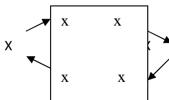
Double Substitution
