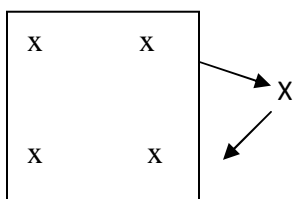
Single Substitution
